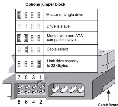
Figure 4 Master/slave jumper settings
