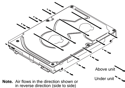
Figure 9. Air flow
