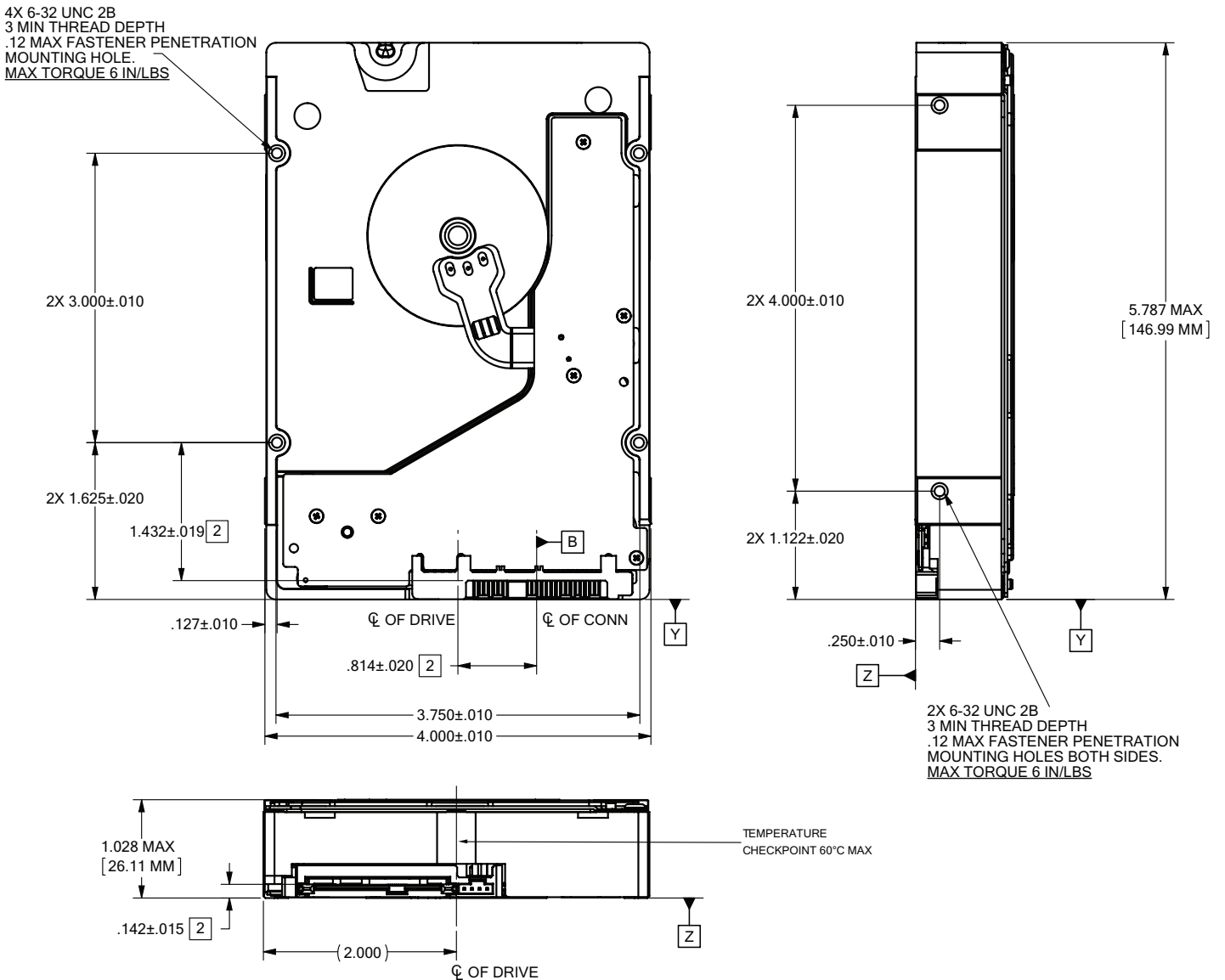
Figure 4. Mounting configuration dimensions (10TB & 8TB)
